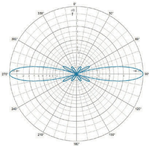
E-Plane | 875 MHz
