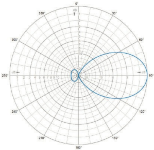
E-Plane | 405 MHz
